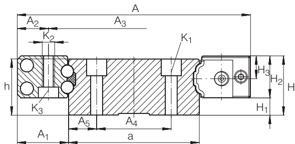
Two KUVS with TKVD 32, TKVD 42 and TKVD 69
