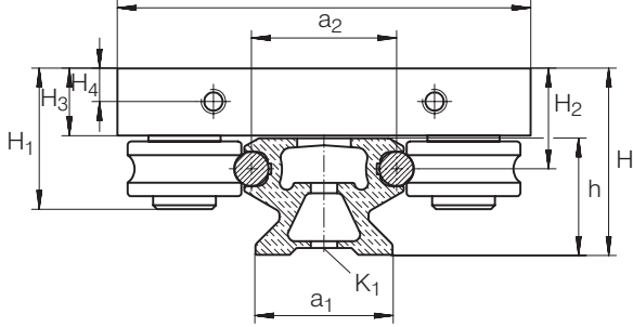
LFL..SF with LFS, LFS..C, LFS..CE
