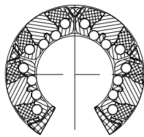
KXO, KXO..PP Main load direction 4)
