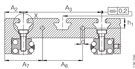
Cross-section of carriages KWVK..AL
