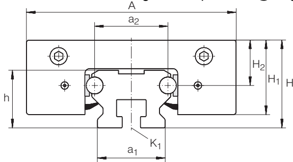
LFKL..SF with LFS..N
