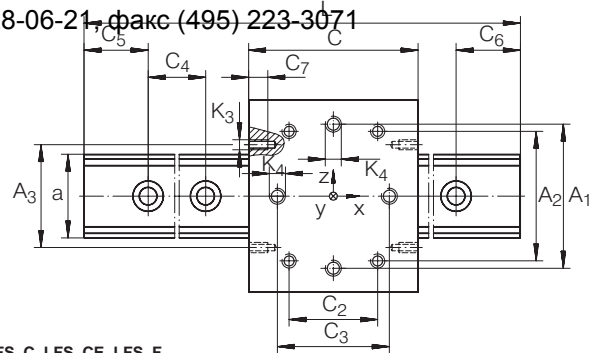
LFL..SF with LFS, LFS..C, LFS..CE, LFS..F, LFS..FE, LFS..N, LFS..NZZ (view rotated through 90°)
