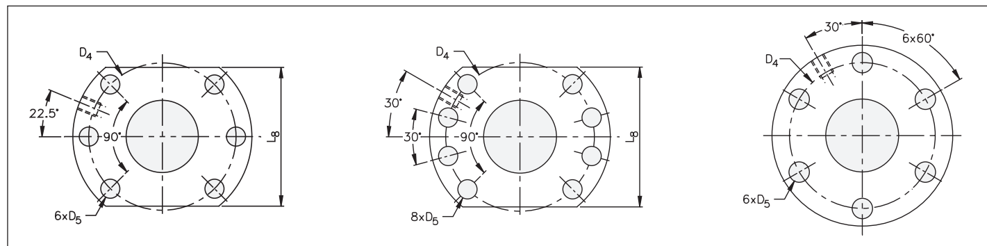
Hole pattern 1
