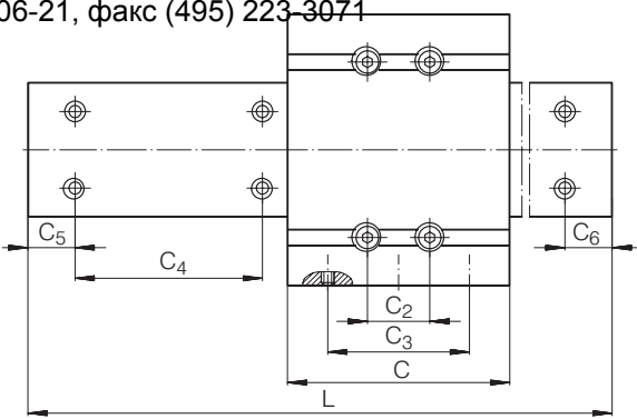
Plan view X (rotated through 90°)
