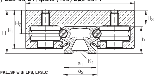
LFKL..SF with LFS, LFS..C
