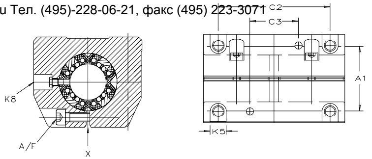
View X (rotated 90°)
