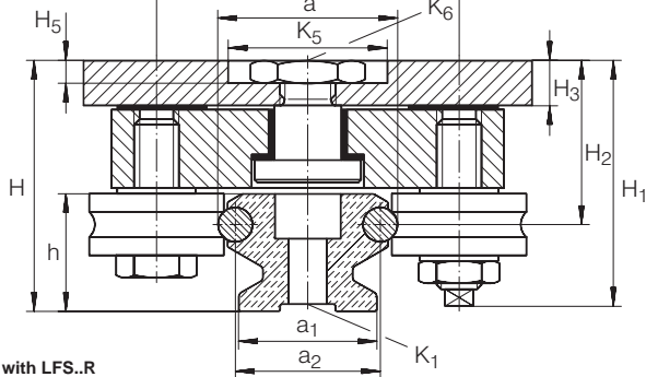
LFDL with LFS..R
