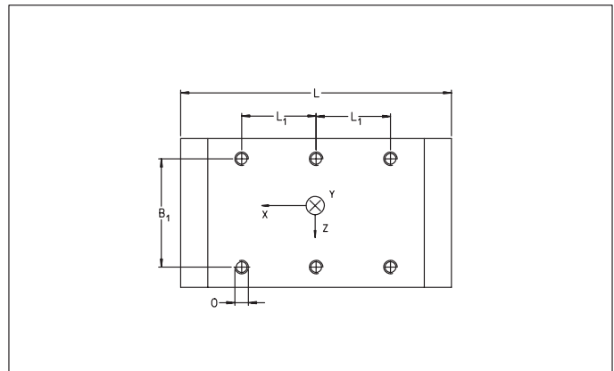
Carriage
