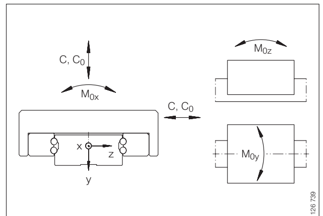
Load directions
