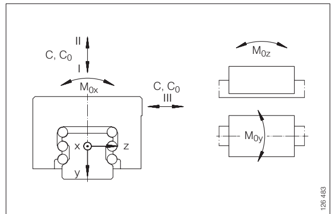
Load directions
