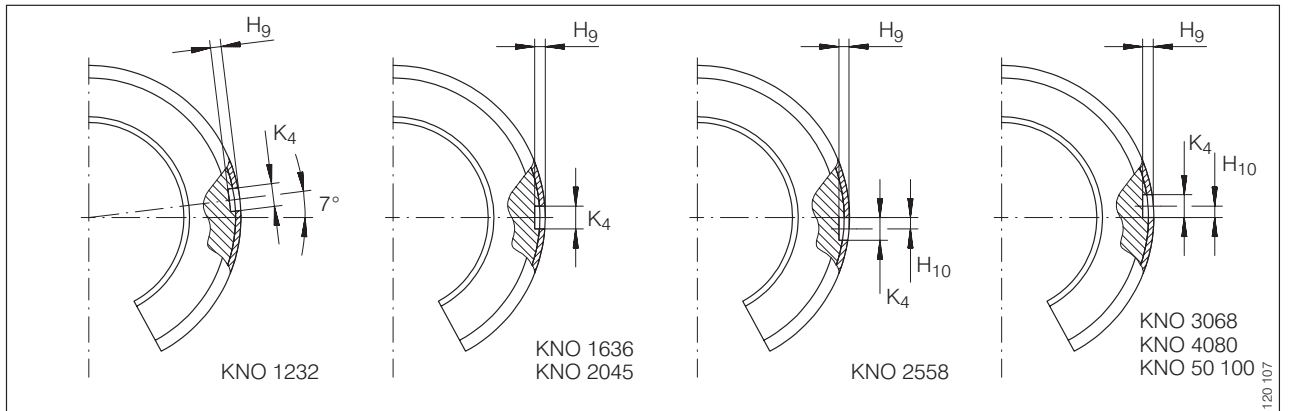
Fixing holes
